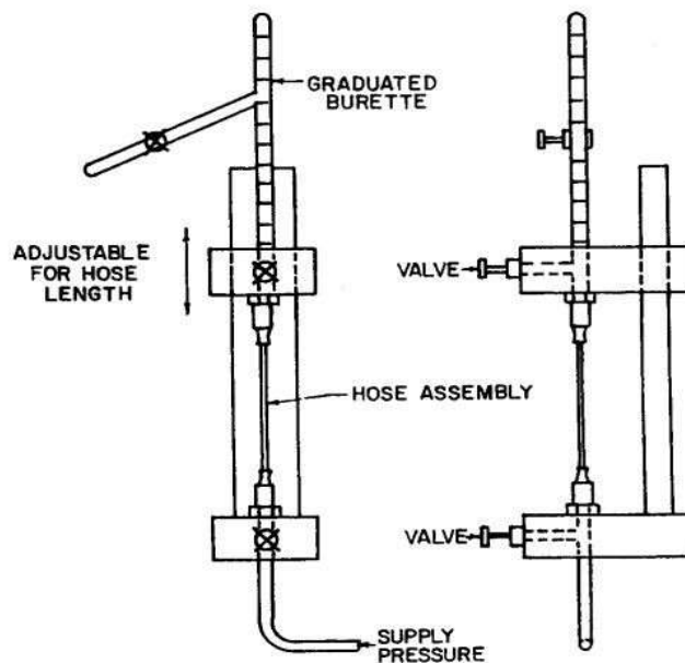
FIGURE 2—EXPANSION TEST APPARATUS
