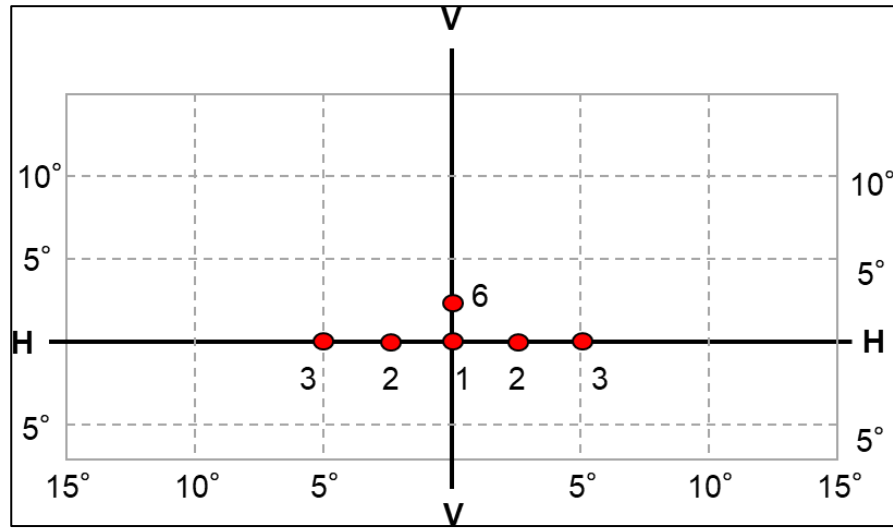
Figure A4-V Passing beam for left-hand traffic
