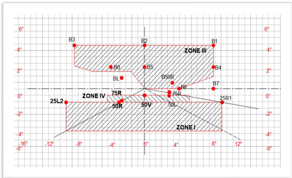
Figure A4-V Passing beam for left-hand traffic
