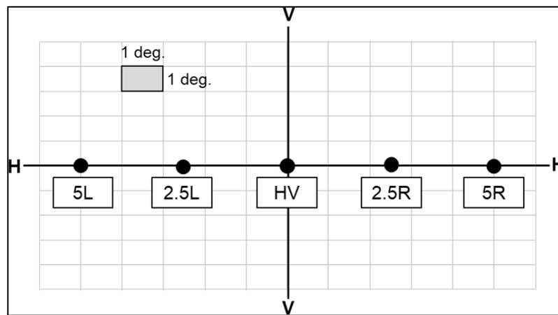
Figure A4-II Driving beam test points
