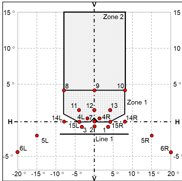
Figure A4-XI Light distribution of the Class F3 front fog lamp
