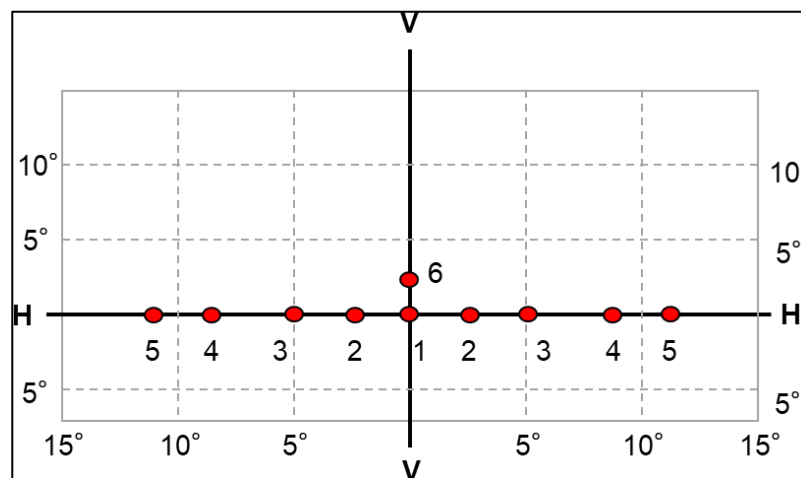
Figure A4-III Primary driving beam - position of test points
