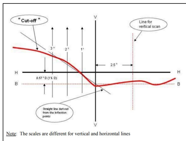
Figure A5-IV Instrumental vertical and horizontal adjustment - Three line scan method
