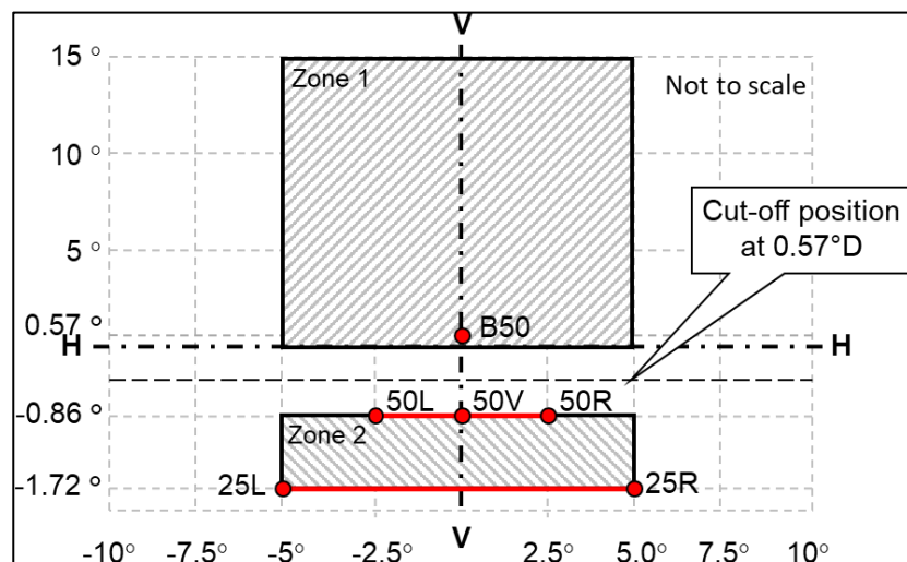
Figure A4-IX Passing beam test points and zones for Class BS headlamp(s)
