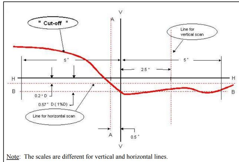
Figure A5-III Instrumental vertical and horizontal adjustment - horizontal line scan method
