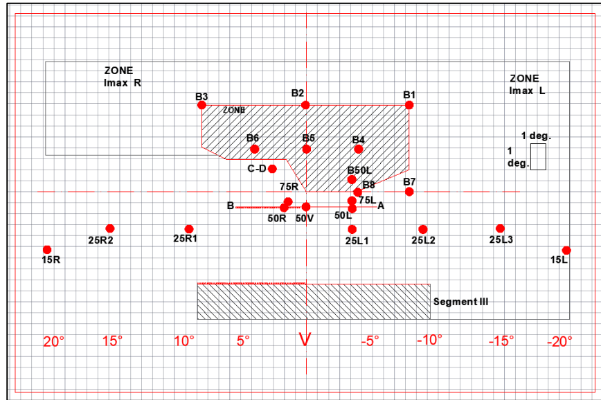
Figure A4-VI Passing beam with gas discharge light sources for left-hand traffic
