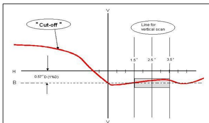
Figure A5-II Measurement of "cut-off" quality
