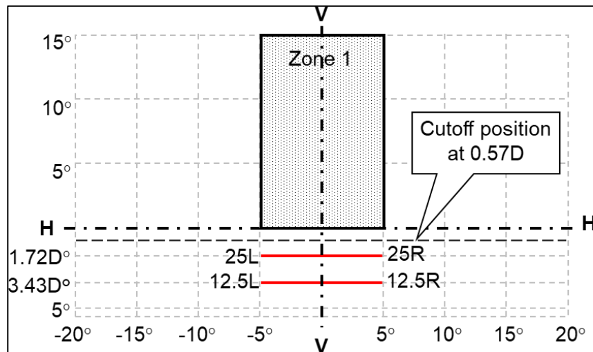
Figure A4-VIII Passing beam test points and zones for Class AS headlamp(s)
