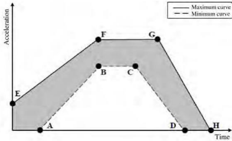
Figure: Generic Description of Test Pulses
