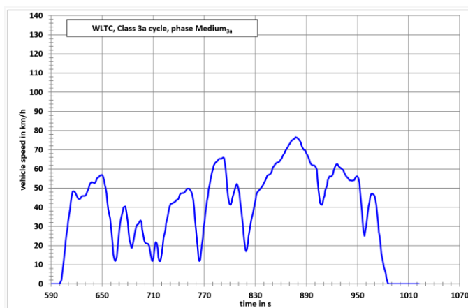
Figure A1/8 WLTC, Class 3a cycle, phase Medium 3a
