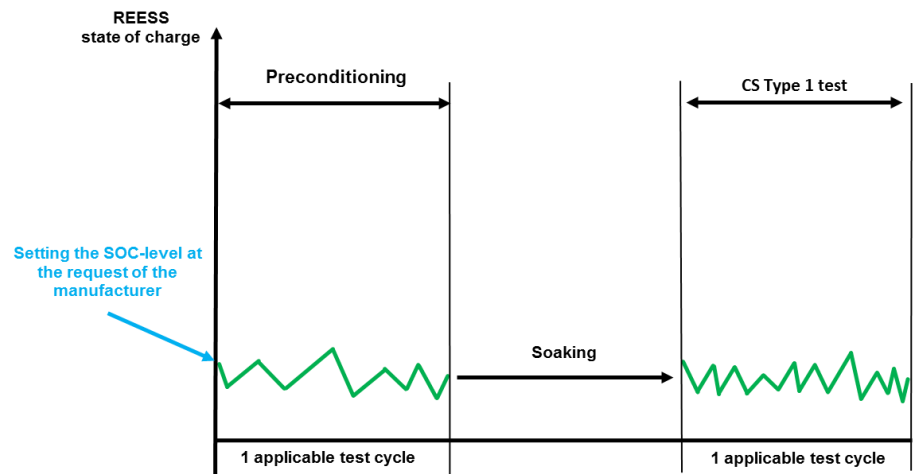
Figure A8.App1/5 NOVC-HEVs and NOVC-FCHVs, charge-sustaining Type I test
