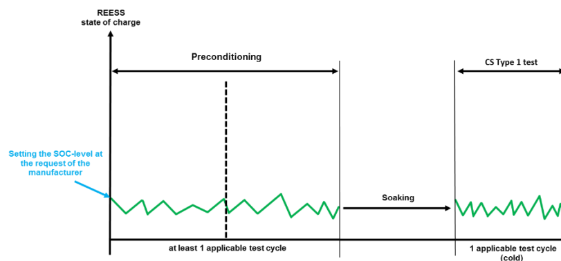
Figure A8.App1/2 OVC-HEVs and OVC-FCHVs, charge-sustaining Type I test
