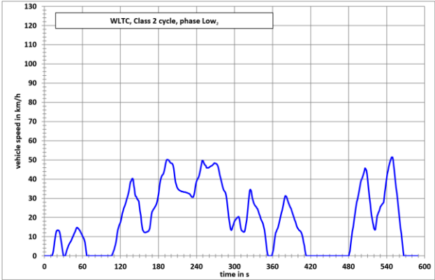
Figure A1/3 WLTC, Class 2 cycle, phase Low 2
