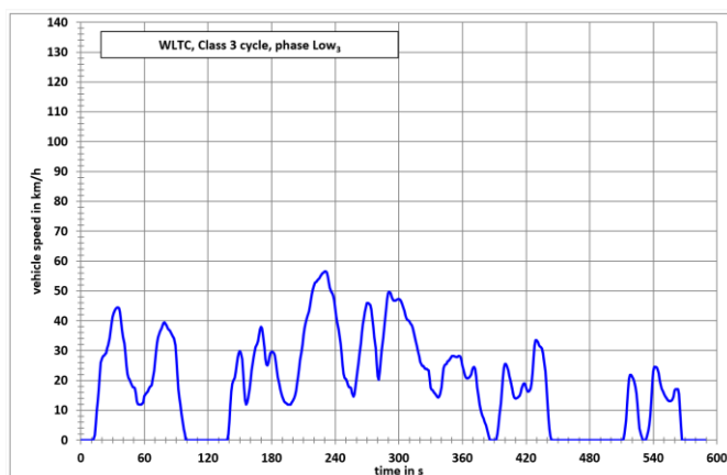
Figure A1/7 WLTC, Class 3 cycle, phase Low 3
