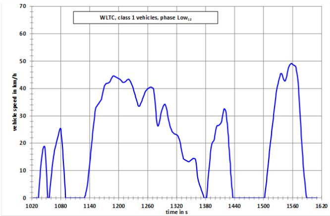
Figure A1/2b WLTC, Class 1 cycle, phase Low 12
