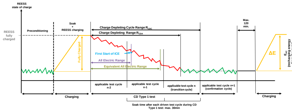
Figure A8.App1/1 OVC-HEVs, charge-depleting Type I test
