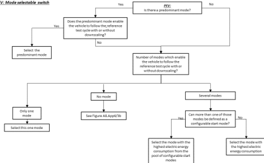
Figure A8.App6/3a PEV: Mode selectable switch
