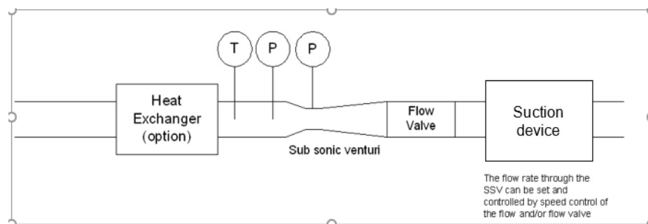
Figure A5/4 Schematic of a subsonic venturi tube (SSV)
