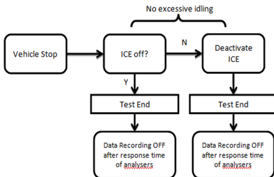
Figure 5 Test end definition
