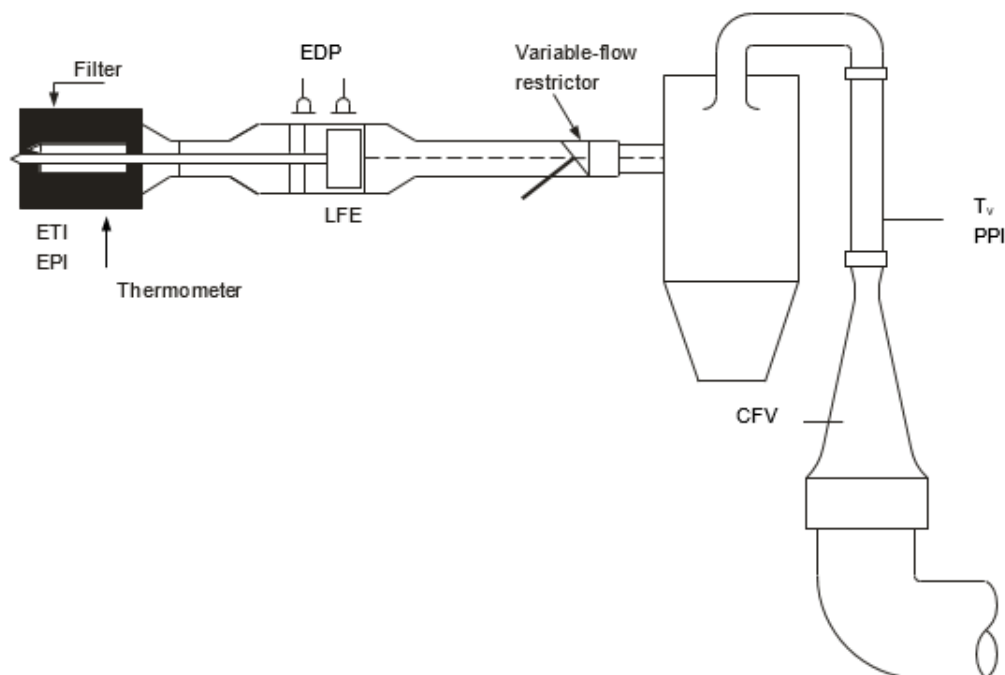
Figure A5/7 CFV calibration configuration
