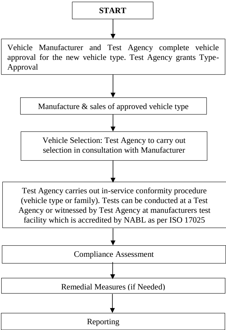
Figure C7/1 Illustration of the In-service Conformity Process
