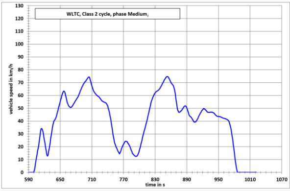
Figure A1/4 WLTC, Class 2 cycle, phase Medium 2
