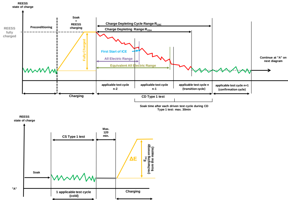
Figure A8.App1/3 OVC-HEVs and OVC-FCHVs, charge-depleting Type I test with subsequent charge-sustaining Type I test
