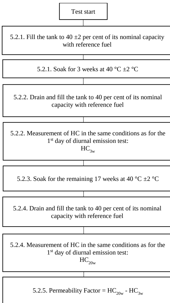
Figure C3/3 Determination of PF
