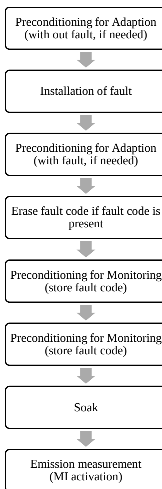
Figure C5.App1/1 Overview of demonstration test
