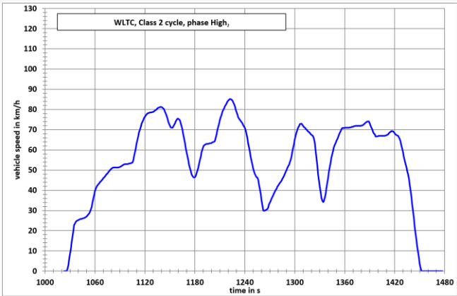
Figure A1/5 WLTC, Class 2 cycle, phase High 2
