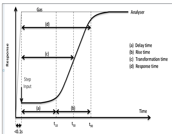
Figure 2 Definition of delay, rise, transformation and response times
