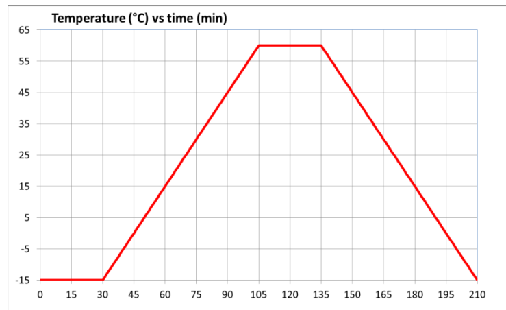
Figure C3/2 Temperature conditioning cycle
