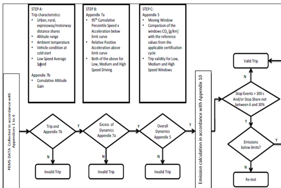
Figure 6 Assessment of trip validity
