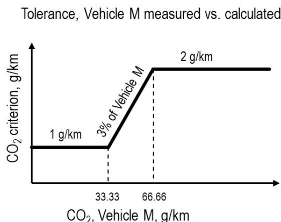
Figure A8/6 Linearity criterion for vehicle M
