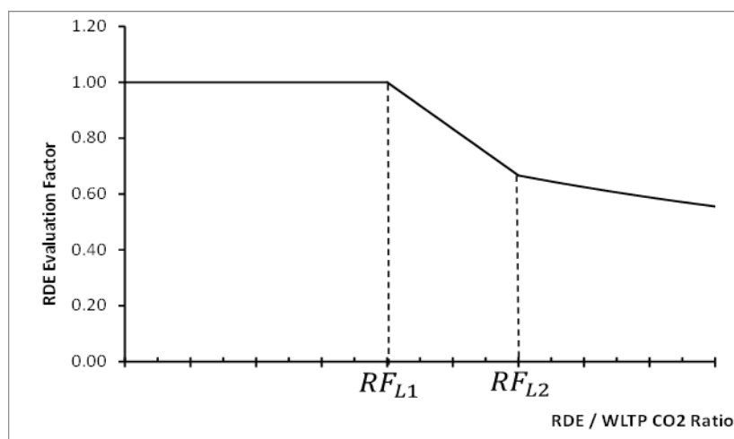
Figure A11/1 Function to calculate the result evaluation factor
