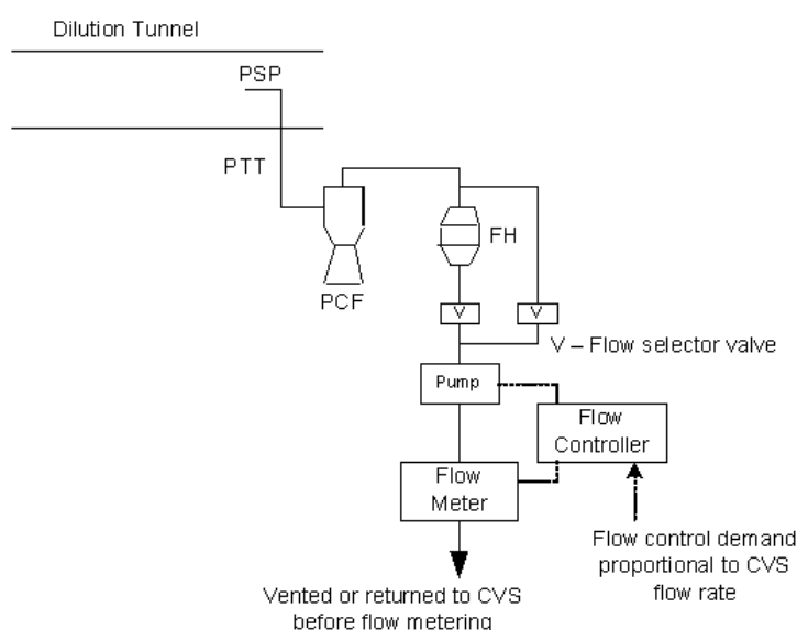
Figure A5/12 Particulate sampling system
