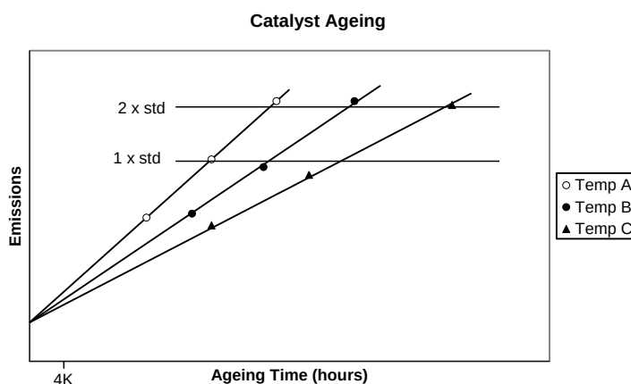
Figure A12 App1/3 Example of catalyst ageing
