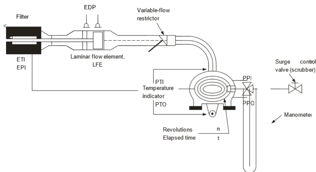
Figure A5/6 PDP calibration configuration
