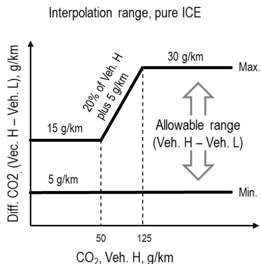
Figure A6/2 Interpolation range for pure ICE vehicles
