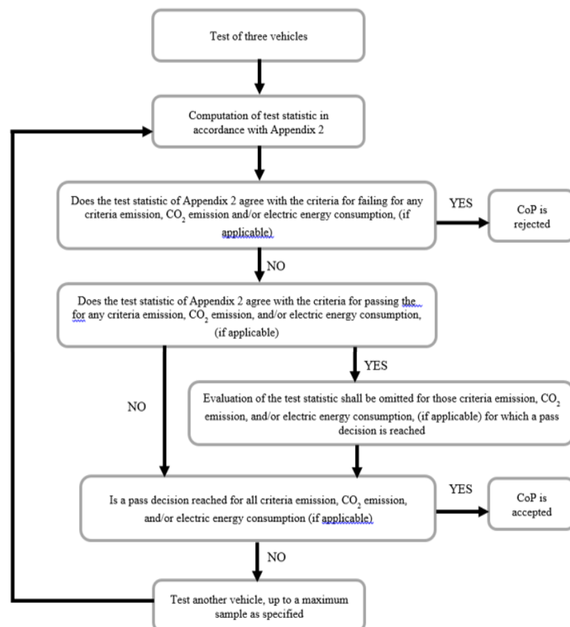
Figure 8/1 Flowchart of the CoP test procedure for the Type I test
