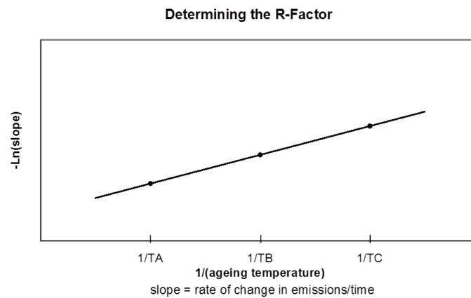
Figure A12 App1/4 Determining the R-Factor
