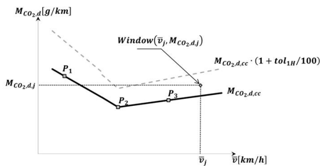
Figure 4: Vehicle CO2 characteristic curve and tolerances for OVC-HEV vehicles (Illustrated for the case
