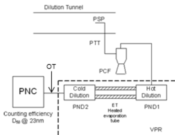
Figure A5/14 A recommended particle sampling system
