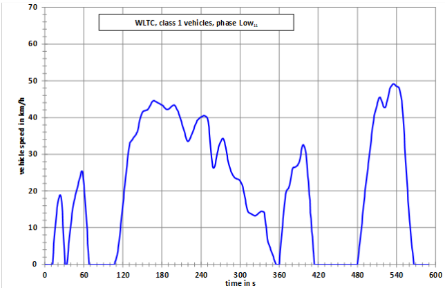
Figure A1/1 WLTC, Class 1 cycle, phase Low 11
