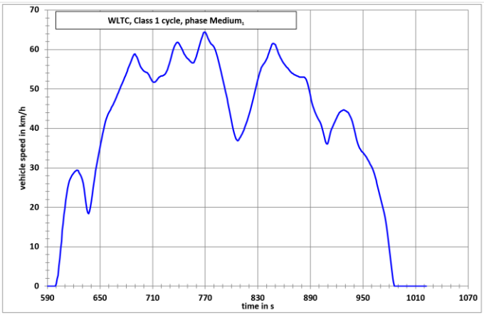
Figure A1/2a WLTC, Class 1 cycle, phase Medium 1
