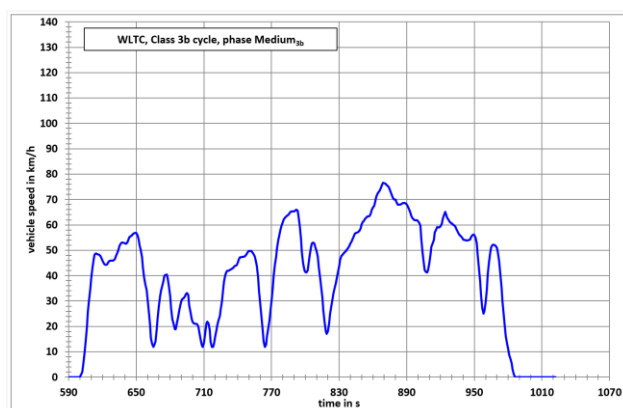
Figure A1/9 WLTC, Class 3b cycle, phase Medium 3b
