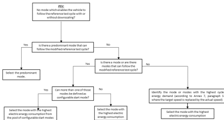
Figure A8.App6/3b PEV: Mode selectable switch
