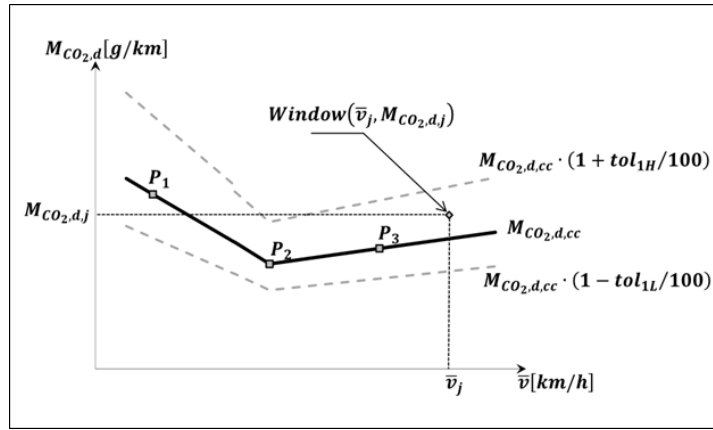
Figure 3 Vehicle CO2 characteristic curve and tolerances for ICE and NOVC-HEV vehicles(Illustrated for the case
