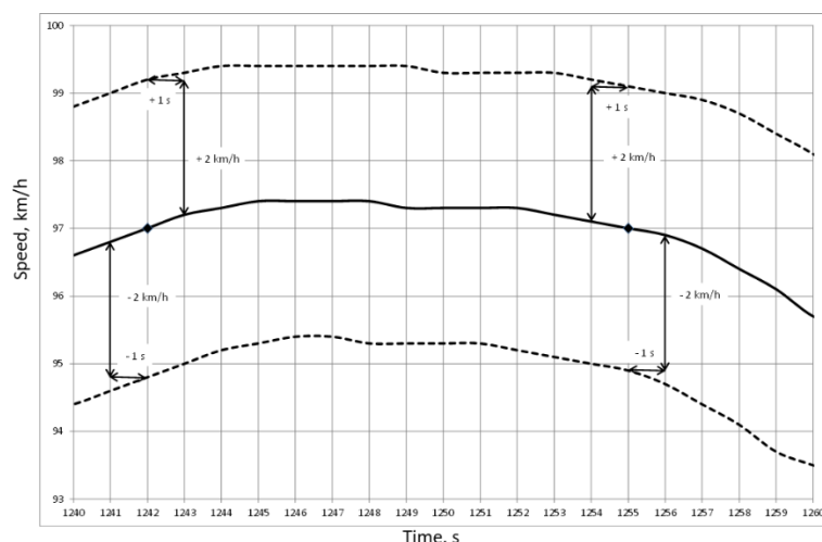
Figure A6/6 Speed trace tolerances
