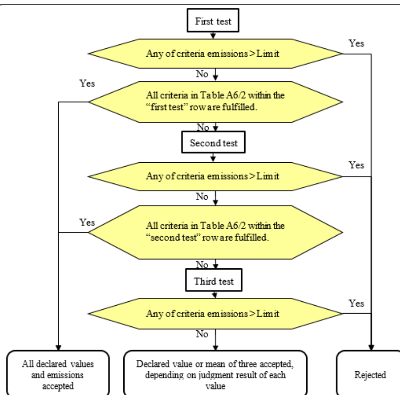
Figure A6/1 Flowchart for the number of Type I tests
