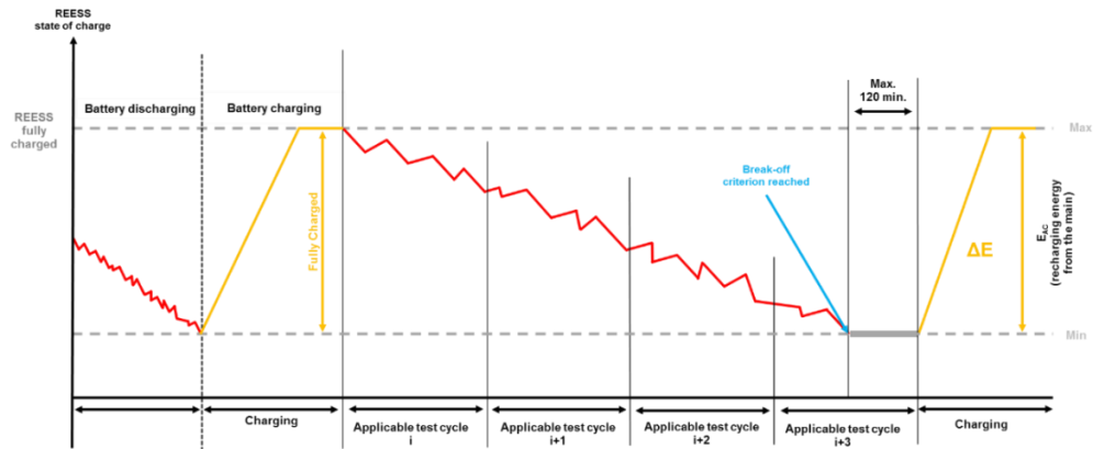
Figure A8.App1/6 Consecutive cycles test sequence PEV
