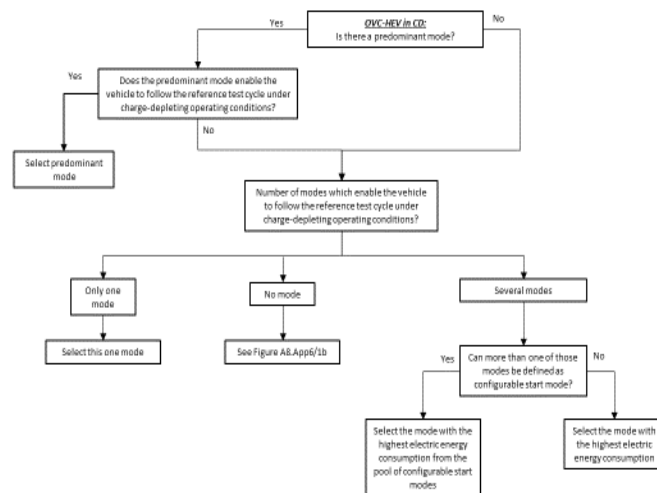
Figure A8.App6/1a OVC-HEV: CD Type 1 Test – Mode selectable switch
