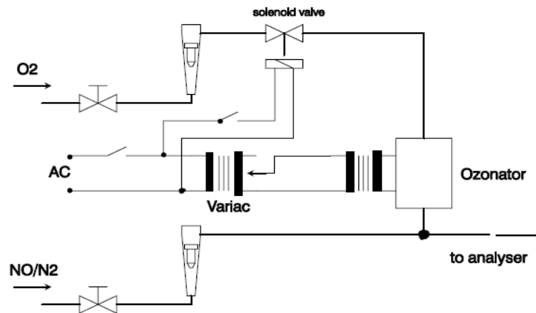
Figure A5/15 NO x converter efficiency test configuration
