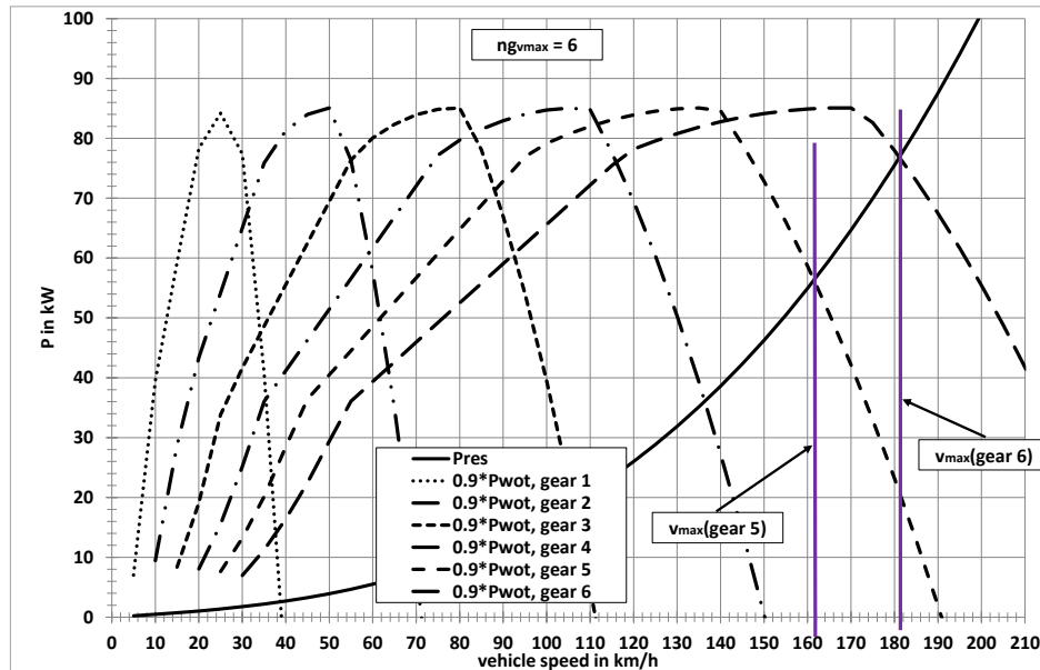
Figure A2/1a An example where ng_{vmax} is the highest gear
