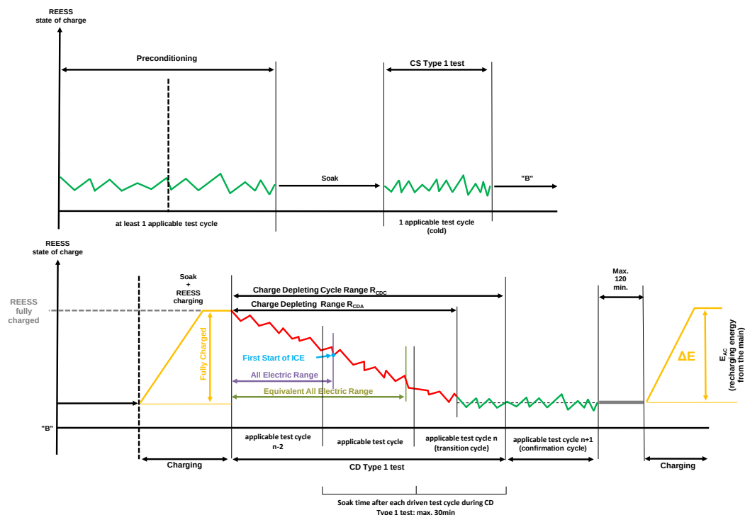
Figure A8.App1/4 OVC-HEVs and OVC-FCHVs, charge-sustaining Type I test with subsequent charge-depleting Type I test
