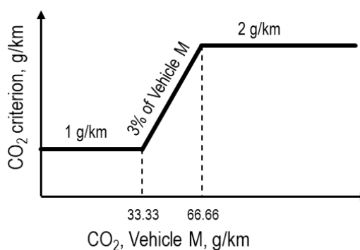
Figure A6/5 Linearity criterion for vehicle M
