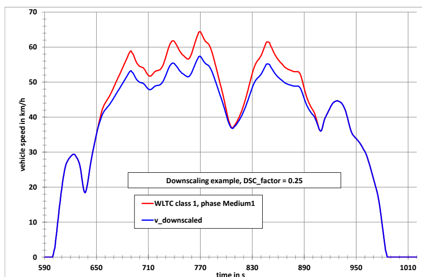
Figure A1/14 Downscaled medium speed phase of the Class 1 WLTC
