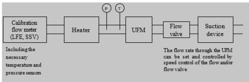
Figure A5/8 UFM calibration configuration
