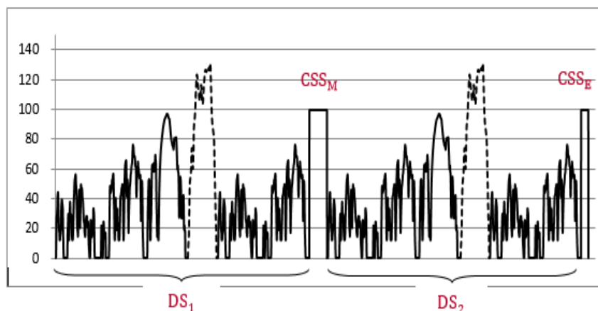
Figure A8/2 Shortened Type I test procedure speed trace
