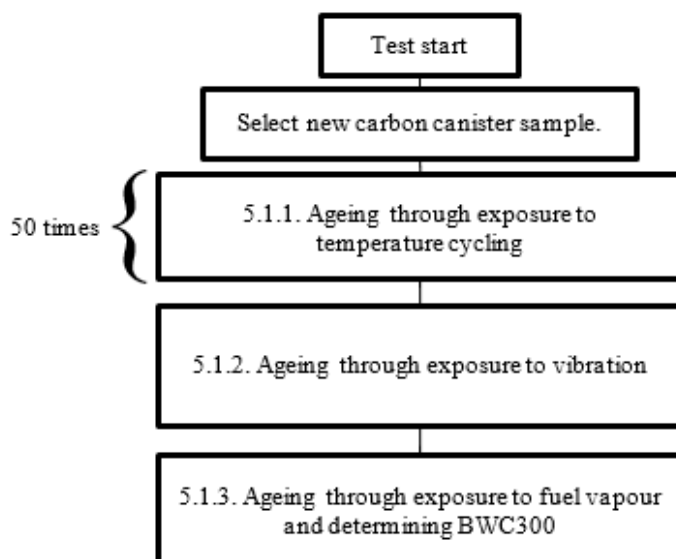
Figure C3/1 Carbon canister bench ageing procedure
