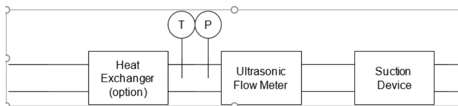
Figure A5/5 Schematic of an ultrasonic flow meter (UFM)
