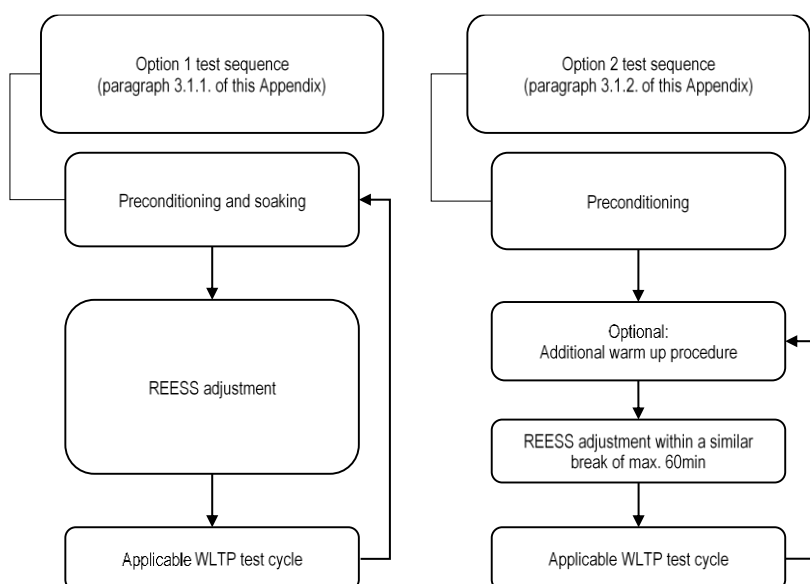
Figure A8.App2/1 OVC-HEV, and OVC-FCHVs test sequences
