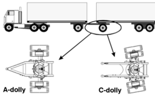
Converter dolly
