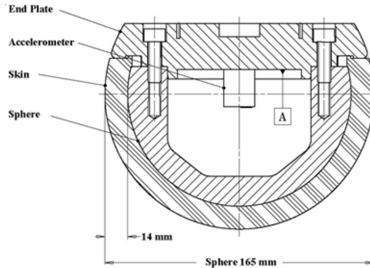
Figure 23 Child Headform Impactor
