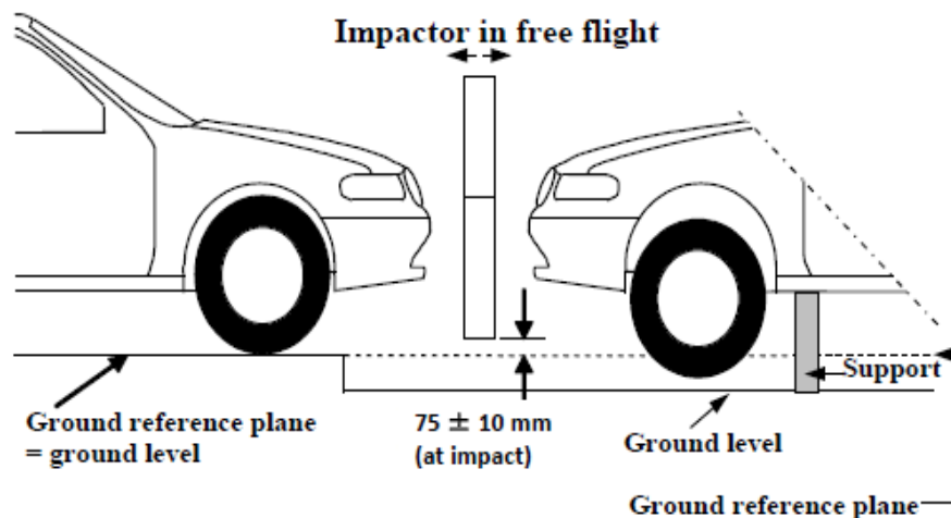
Figure 26 Lower Legform to Bumper Tests for Complete Vehicle in Normal Ride Attitude (Left) and for Cut-Body Mounted on Supports (Right)
