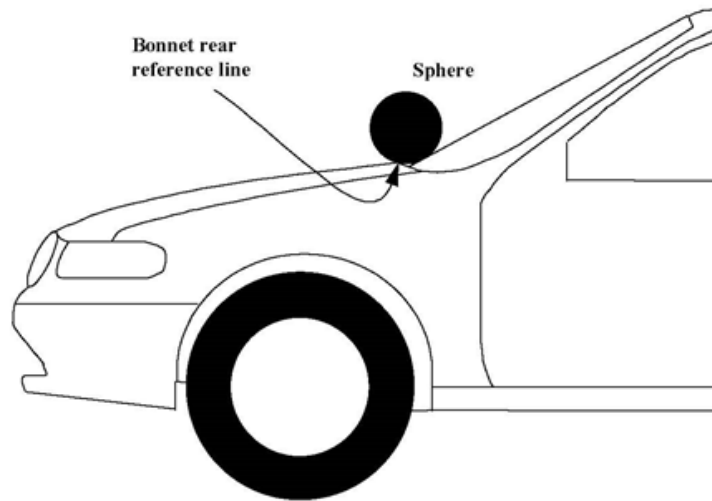
Figure 2 Bonnet Rear Reference Line
