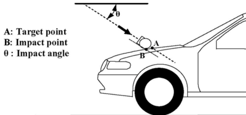
Figure 6 Impact and Target Point
