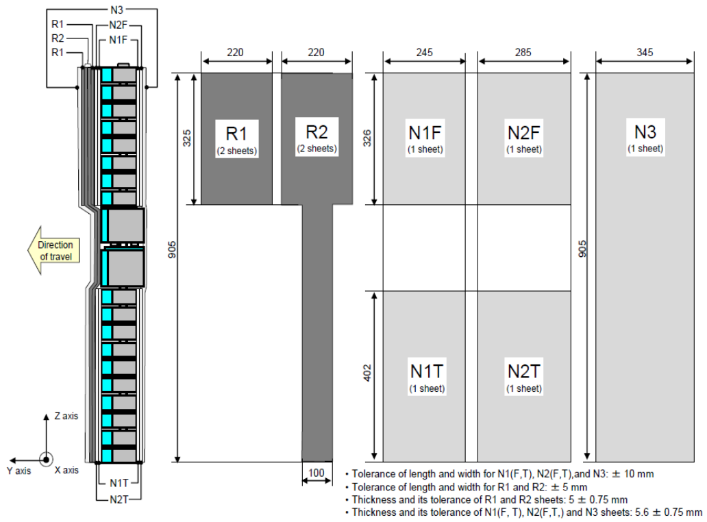
Figure 19 Flexible lower legform impactor: Flesh and skin dimensions
