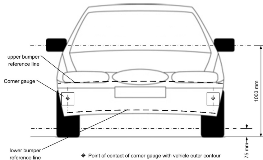
Figure 11 Corner gauge
