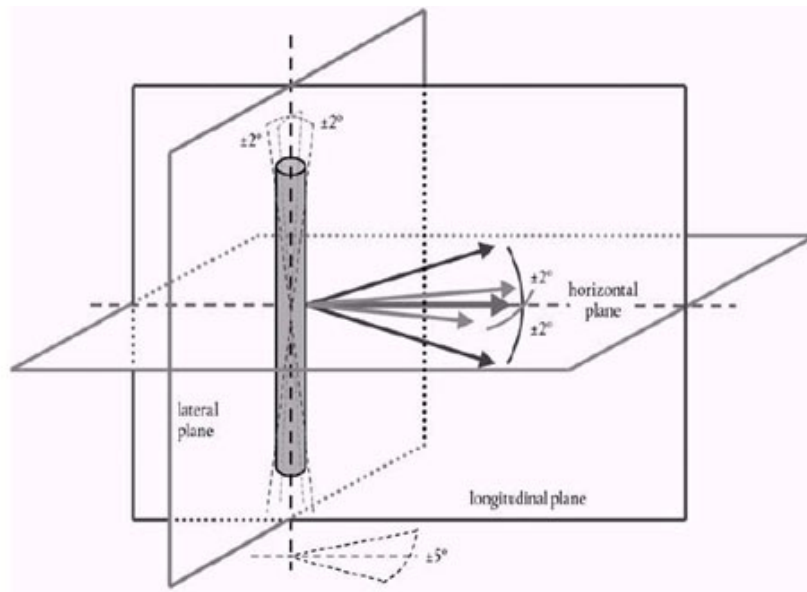
Figure 25 Tolerances of Angles for the Flexible Lower Legform Impactor at the time of the First Impact (see Paragraphs 7.1.1.3 and 7.1.1.6)
