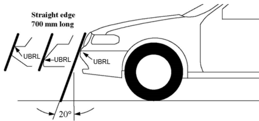
Figure 9 Upper Bumper Reference Line
