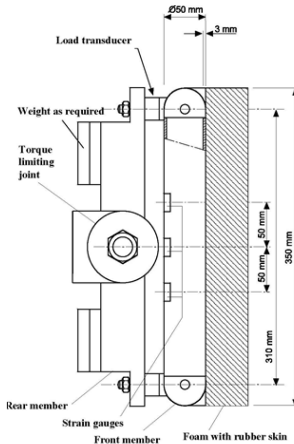
Figure 22 Upper Legform Impactor
