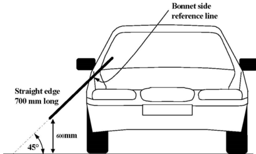
Figure 8 Side Reference Line
