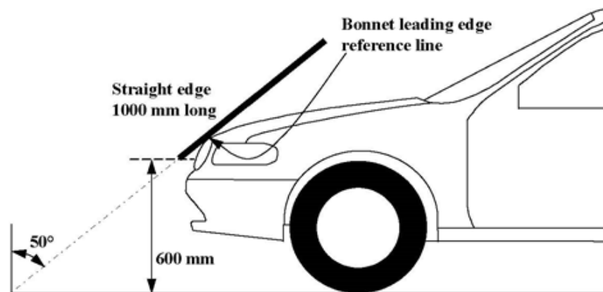
Figure 1 Bonnet Leading Edge Reference Line
