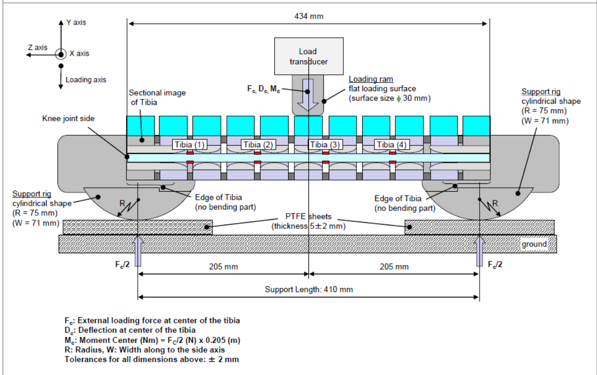
Figure 30 Flexible lower legform impactor: Test set-up for the tibia in the static certification test
