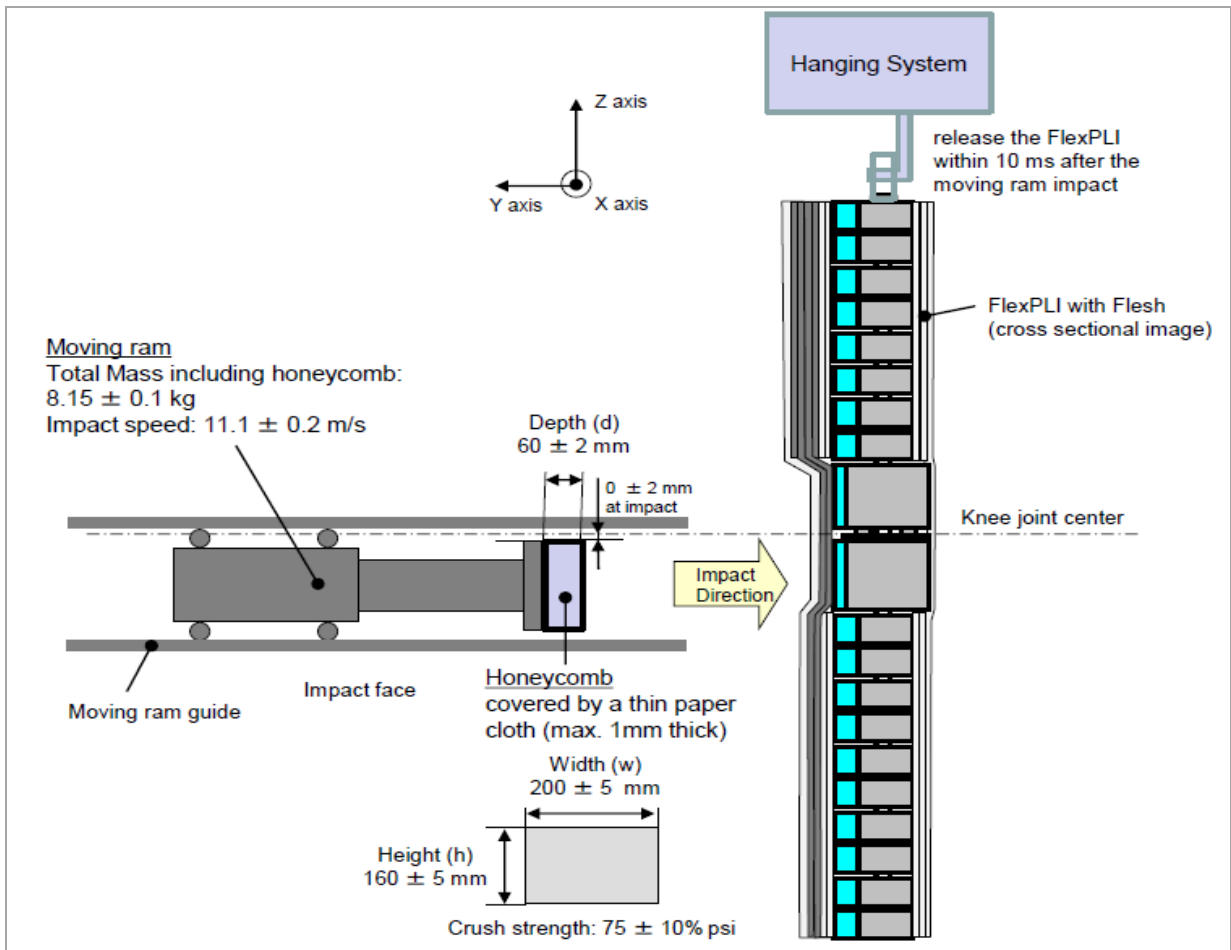
Figure 33 Flexible lower legform impactor: Test set-up for the dynamic lower legform impactor certification test – Inverse Test
