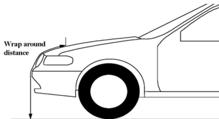
Figure 10 Wrap around Distance Measurement
