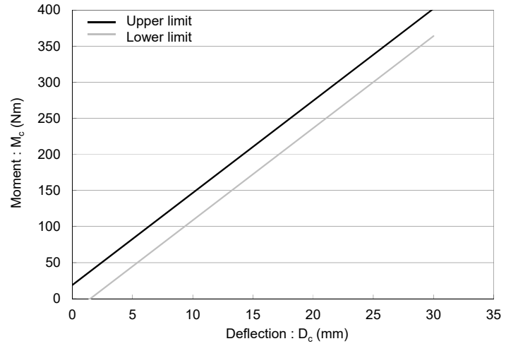
Figure 27 Flexible lower legform impactor: Requirement corridors of the femur and the tibia in the static certification test
