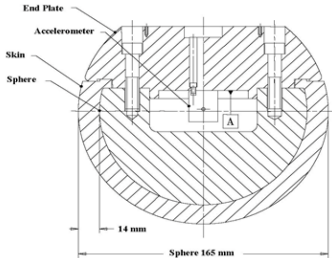
Figure 24 Adult Headform Impactor
