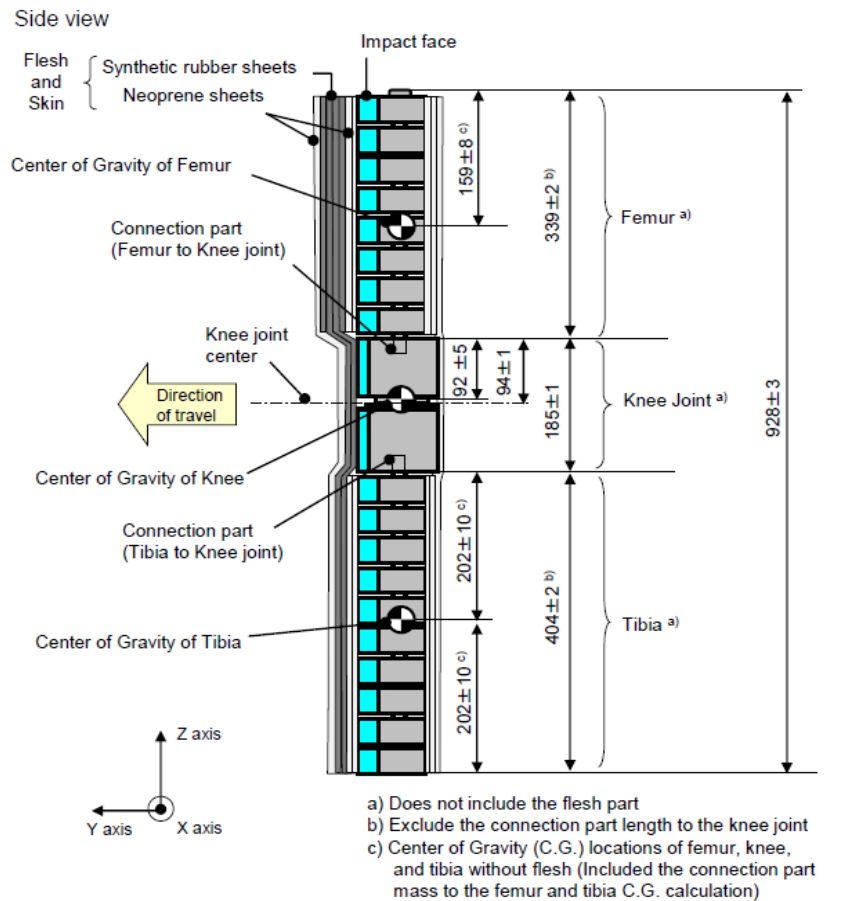
Figure 17 Flexible lower legform impactor Dimensions and center of gravity locations of femur, knee joint and tibia (side view)
