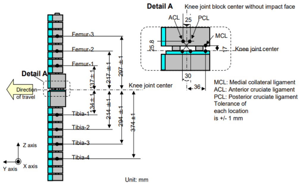
Figure 21 Flexible lower legform impactor instrument locations
