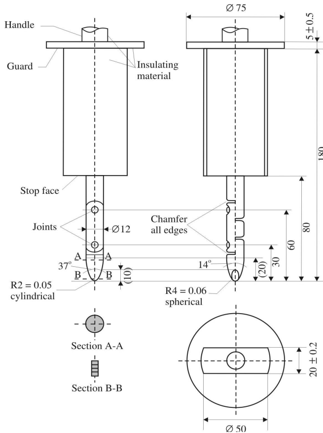
Figure 3 Jointed Test Finger
