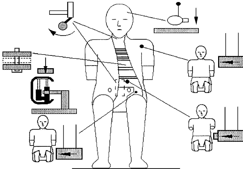
Figure 3 Overview of the Side Impact Dummy Certification Test Set-up
