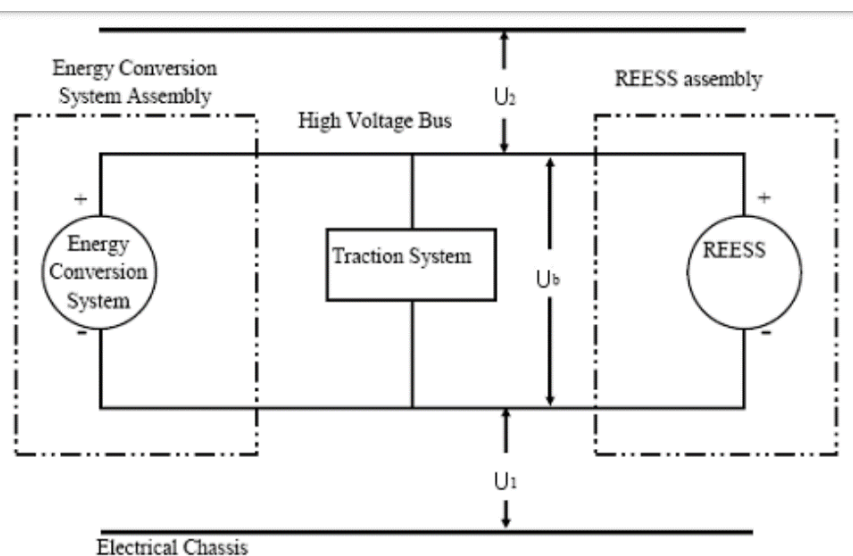
Figure 1 Measurement of U_b , U_1 , U_2
