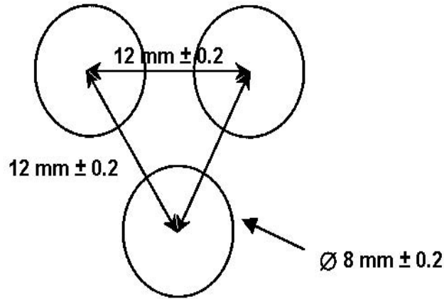
Figure 7 Staggered Pitch for the Back-Plate Ventilation Holes
