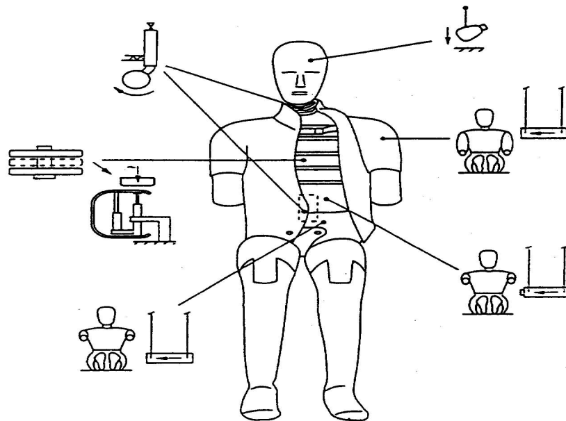
Figure 3 Overview of Dummy Certification Test Set-up
