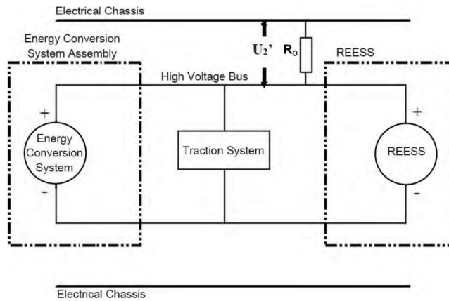
Figure 6 Measurement of U_2'
