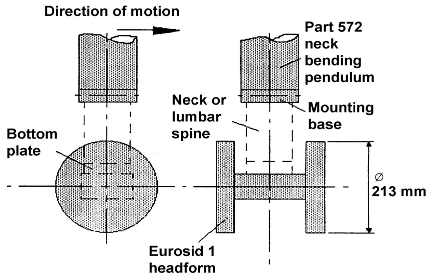
Figure 4 Neck and Lumbar Spine Certification Test Set-up
