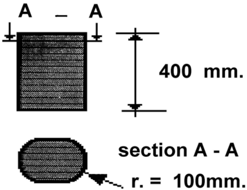
Figure 3 Body Block Impactor
