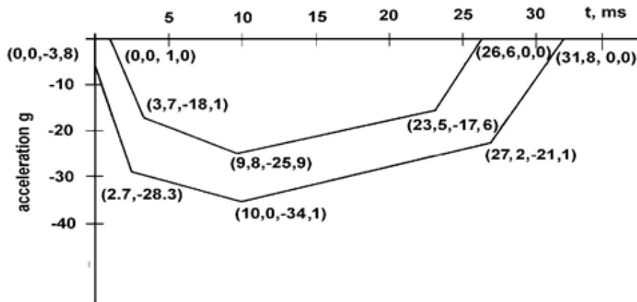
Figure 5 Pendulum Deceleration-time Corridor for Neck Certification Test
