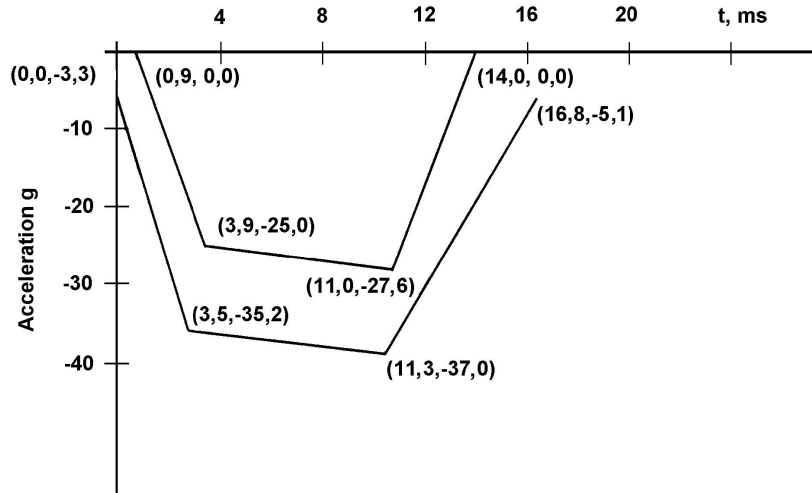
Figure 5 Pendulum Deceleration-time Corridor for Neck Certification Test
