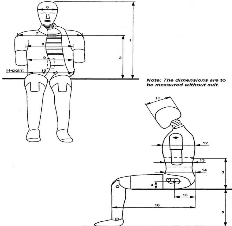
Figure 2 Measurements for Principle Dummy Dimensions (see Table 3)
