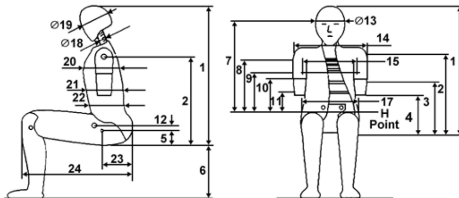
Figure 2 Measurements for Principle Dummy Dimensions
