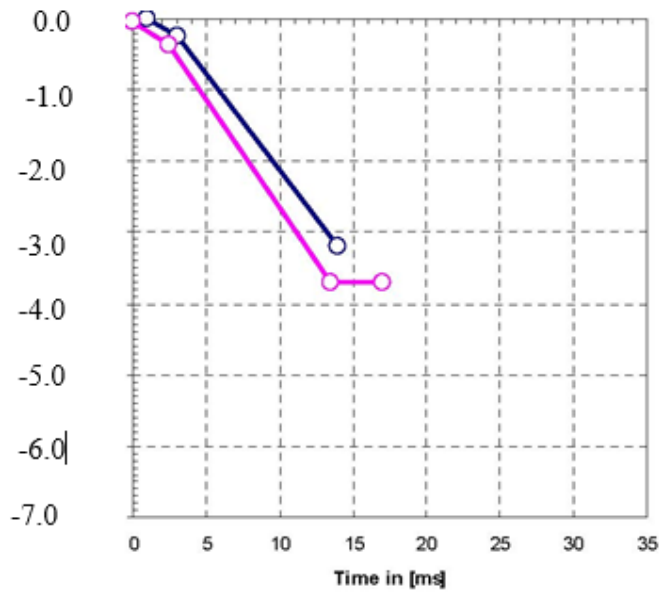
Pendulum velocity change corridor for neck certification
