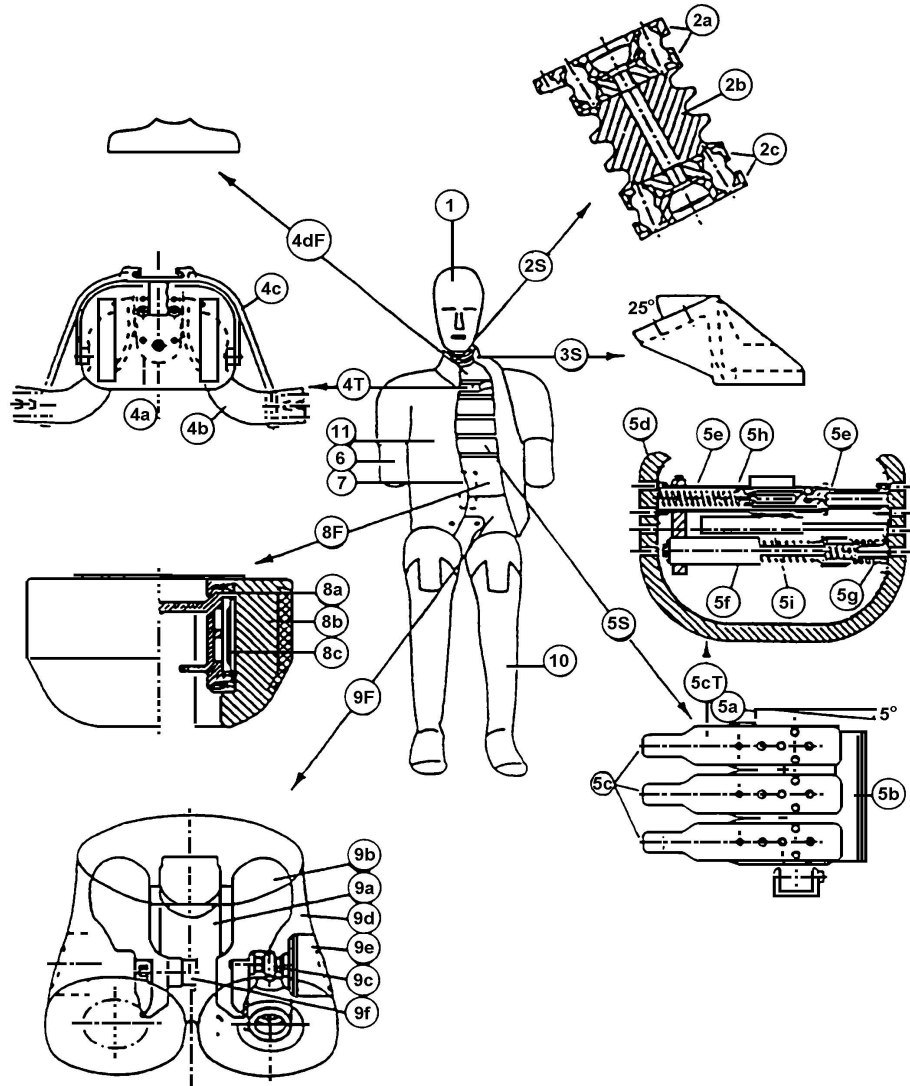
Figure 1 Construction of Side Impact Dummy
