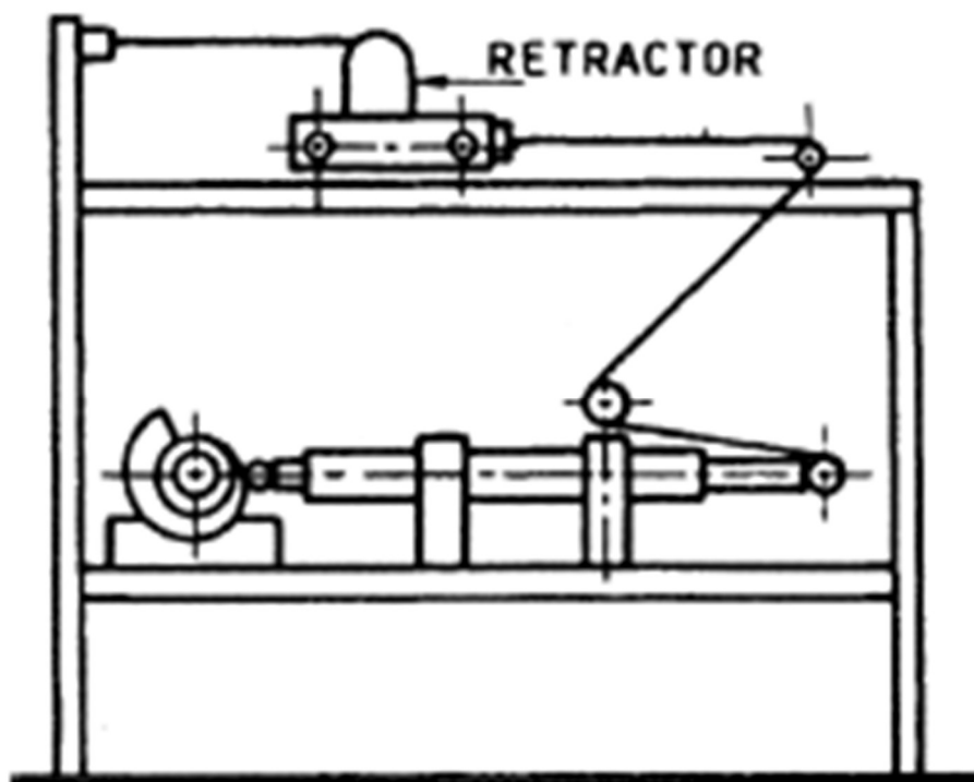
Fig. Typical Apparatus to test Locking of Emergency Locking Retractors
