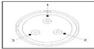
3 PIN LEMO PLUG VIEW FACING PINS LEMO PART NO. FGG.OB.303 CLAD52Z
