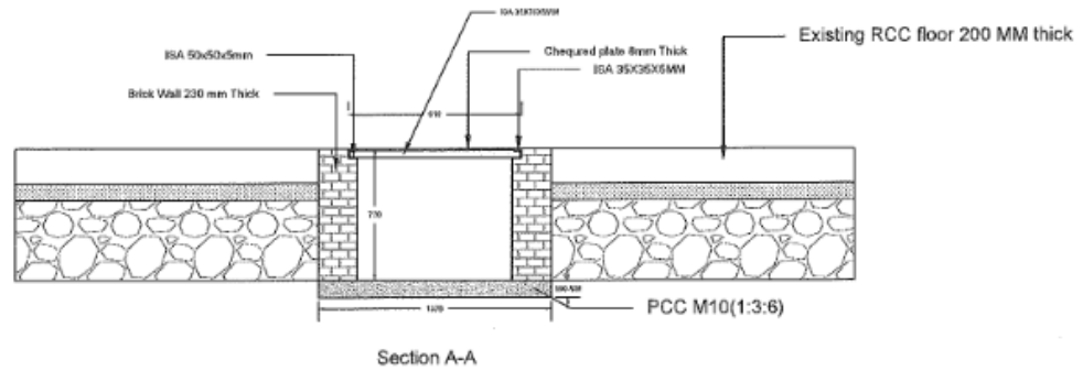
Fig. : B4-Trench Construction on RCC Floor Location-2
