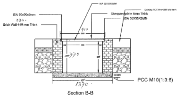
Fig. : B4-Trench Construction on RCC Floor Location-1
